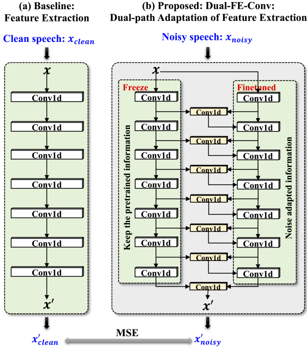
Figure 1: Neural network structure of (a) baseline feature extraction module; (b) proposed dual-path adaptation of feature extraction module (Dual-FE-Conv).
