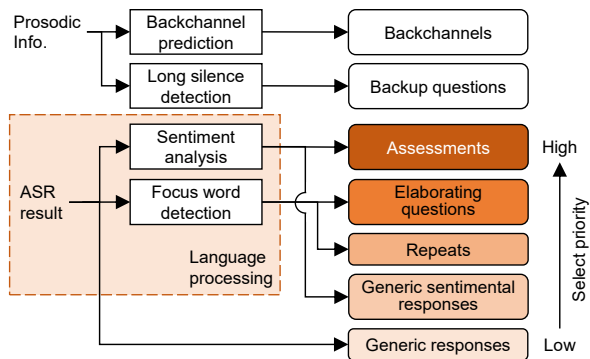
Figure 2: Architecture of listener response generation
